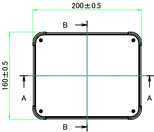
E view
